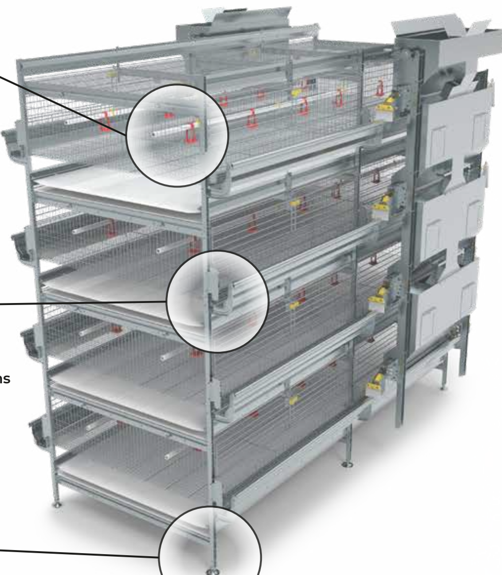
Drinking lines on each floor
